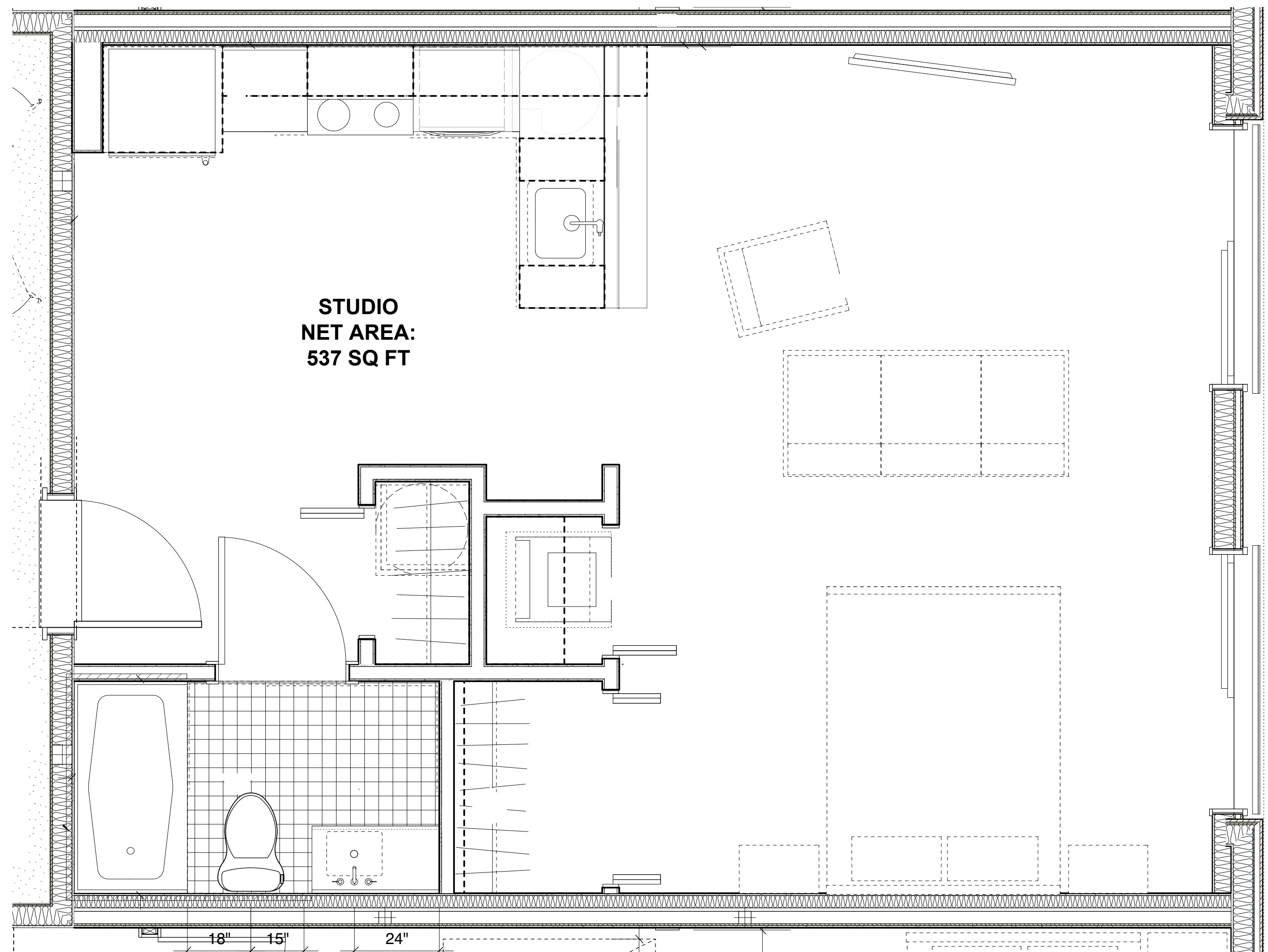
1 UNIT TYPE B - STUDIO, UNITS 101,201 A7.30 SCALE: 1/2" = 1'-0"
