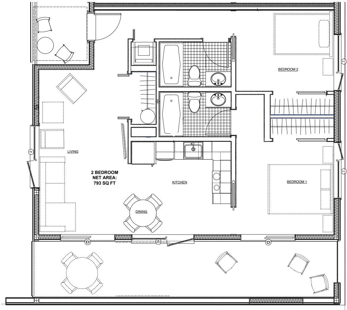
1 A7.4G UNIT TYPE C - 2 BEDROOM, UNITS 301,302,300,302 SCALE: 1/2" = 1'-0"
