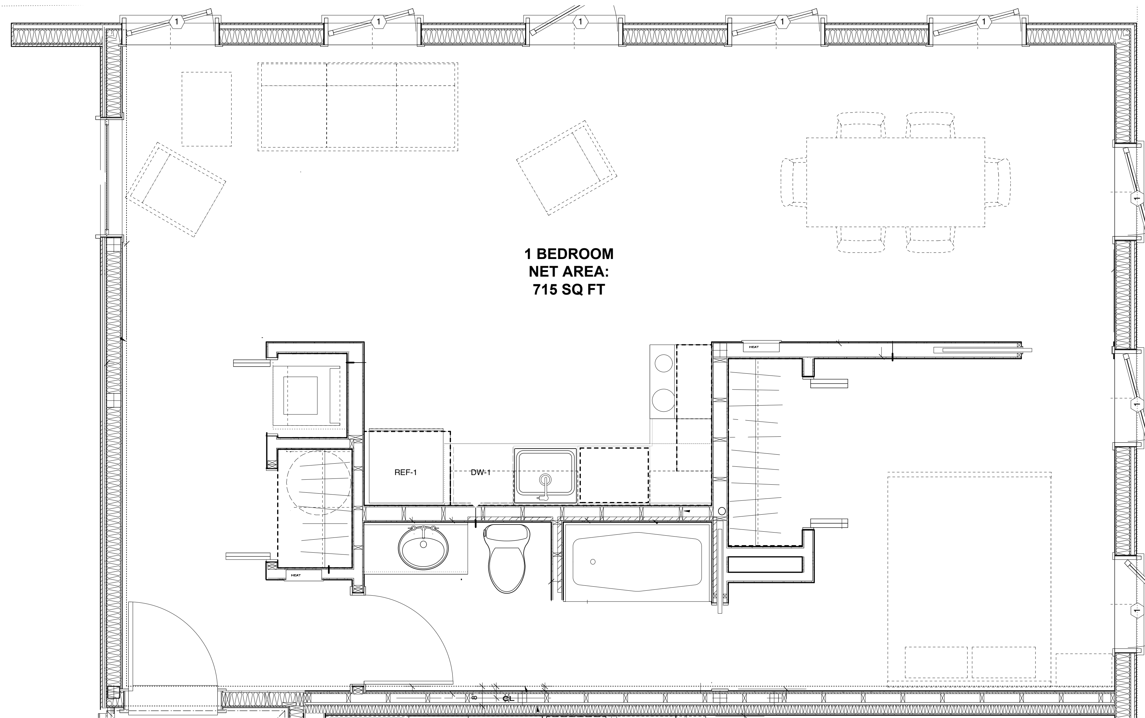
1 UNIT TYPE A1 - 1 BEDROOM, UNITS 100,102, 200,202 A7.10 SCALE: 1/2" = 1'-0"
